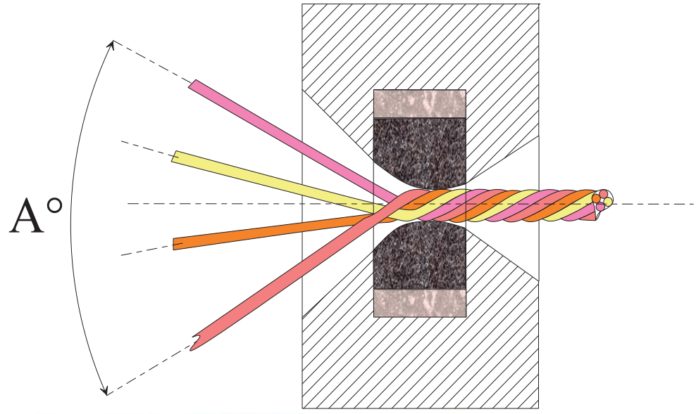
Stranding dies
