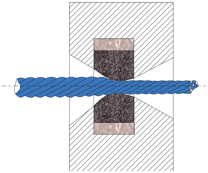
Compacting die
