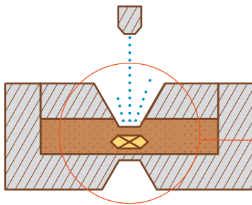
4-Pre-opening
