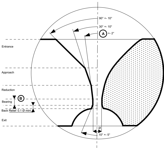
NSCD - SSCD dies Ø up to .002"
