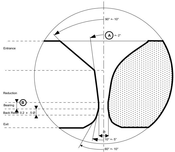
NSCD - SSCD dies Ø .002" to .004"
