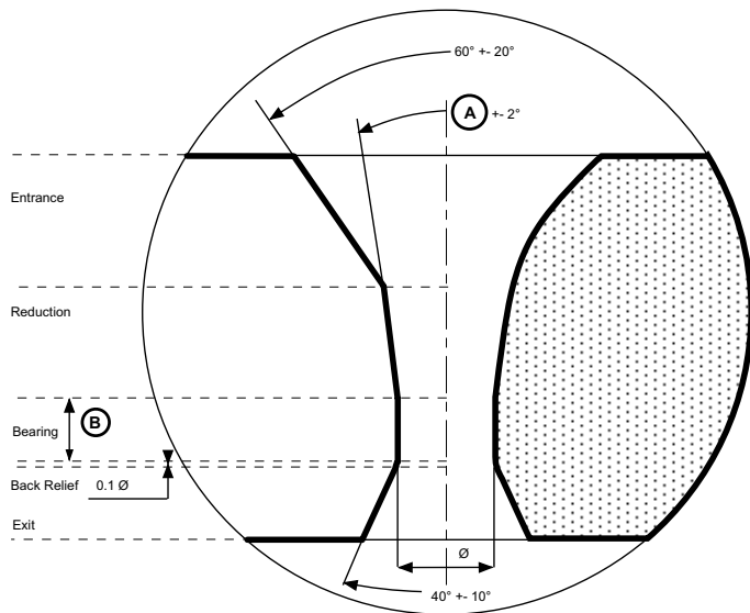
NSCD - SSCD dies Ø over .004"
